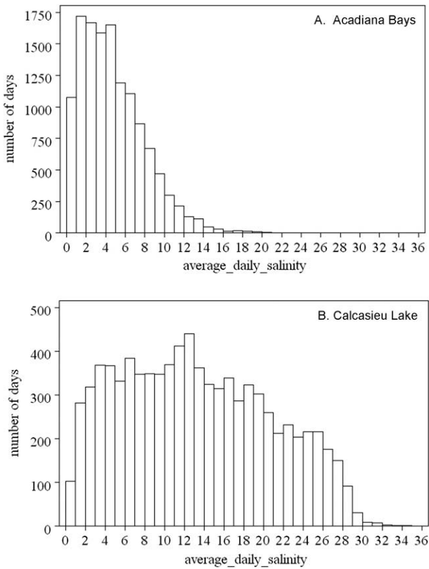
Fig. 5. Distribution of mean daily water salinity in marshes of the Acadiana Bays (A) and of Calcasieu Lake (B), Louisiana, USA. Mean daily water salinity was calculated from 521,561 hourly observations.
