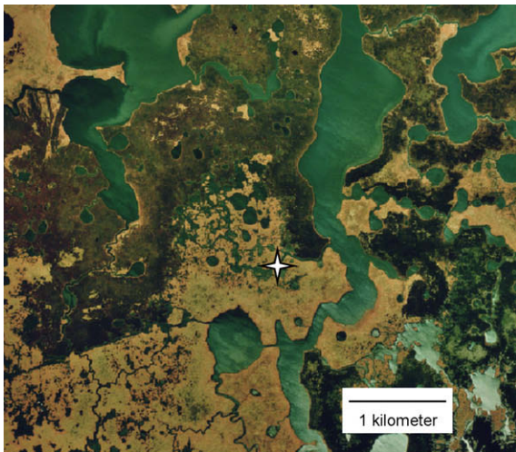
Fig. 2. Portion of a Digital Orthophoto Quarter Quadrangle from 1998 showing a wetland landscape that typifies coastal Louisiana. Topography across the area pictured varies less than 30 cm in marsh areas (i.e., supporting emergent vegetation), and less than 1 m in large open water areas. Only in small tidal channels does topography vary more than 1 m. The star near the center of the figure shows the location of one (MI-Lucien in Tables 1 and 2) of the 14 stations where a sensor recorded water level and salinity hourly. At this station, the sensor was in a small tidal channel that was approximately 10 m wide and 3 m deep. Marsh elevation was measured within 60 m of sensor at this and all other stations. The virtually flat landscape, the short distance between the sensor, and a daily tidal range averaging 26 cm prevents slopes in water surface elevation between sensor and marsh that would introduce error into estimates of flooding depth and duration.
