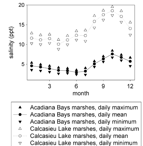
Fig. 9. Monthly variability in daily maximum salinity, daily mean salinity, and daily minimum salinity of water in marshes of the Acadiana Bays and of Calcasieu Lake, Louisiana, USA.
