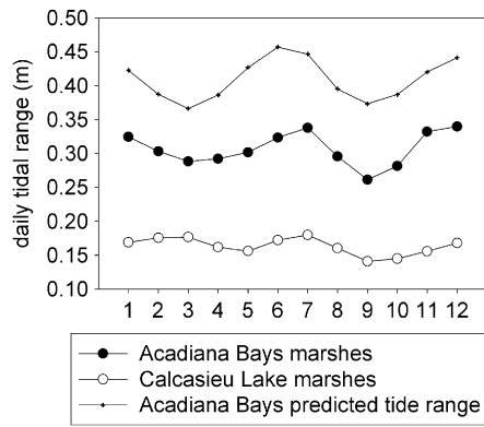
Fig. 10. Monthly variability in daily tidal range based on predicted water levels from NOAA Station number 8765251 (Cypremort Point), and based on observed water levels in marshes of the Acadiana Bays and of Calcasieu Lake, Louisiana, USA.
