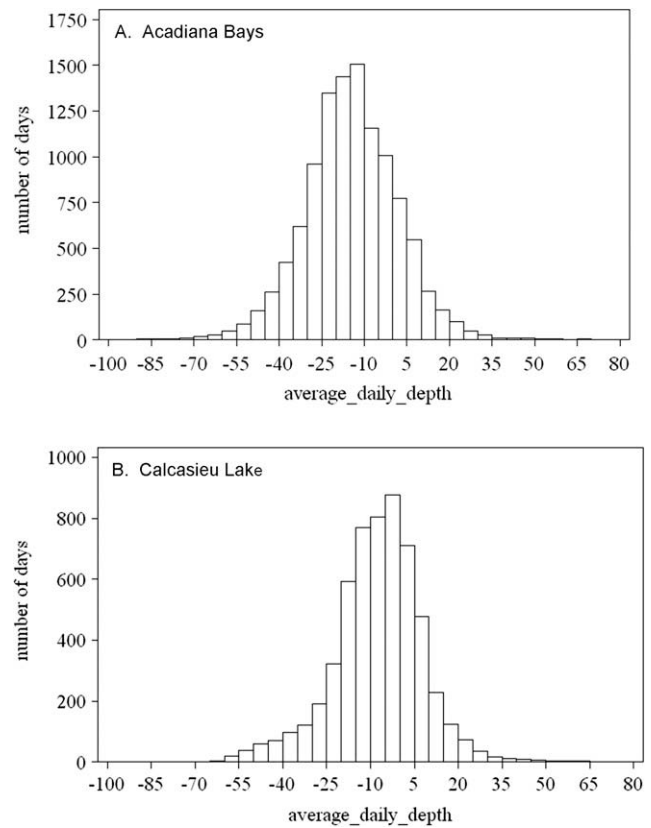
Fig. 4. Distribution of mean daily water depth in marshes of the Acadiana Bays (A) and of Calcasieu Lake (B), Louisiana, USA. Mean daily water depth was calculated from 399,772 hourly observations.
