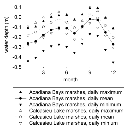
Fig. 8. Monthly variability in daily maximum depth, daily mean depth, and daily minimum depth of water in marshes of the Acadiana Bays and of Calcasieu Lake, Louisiana, USA.
