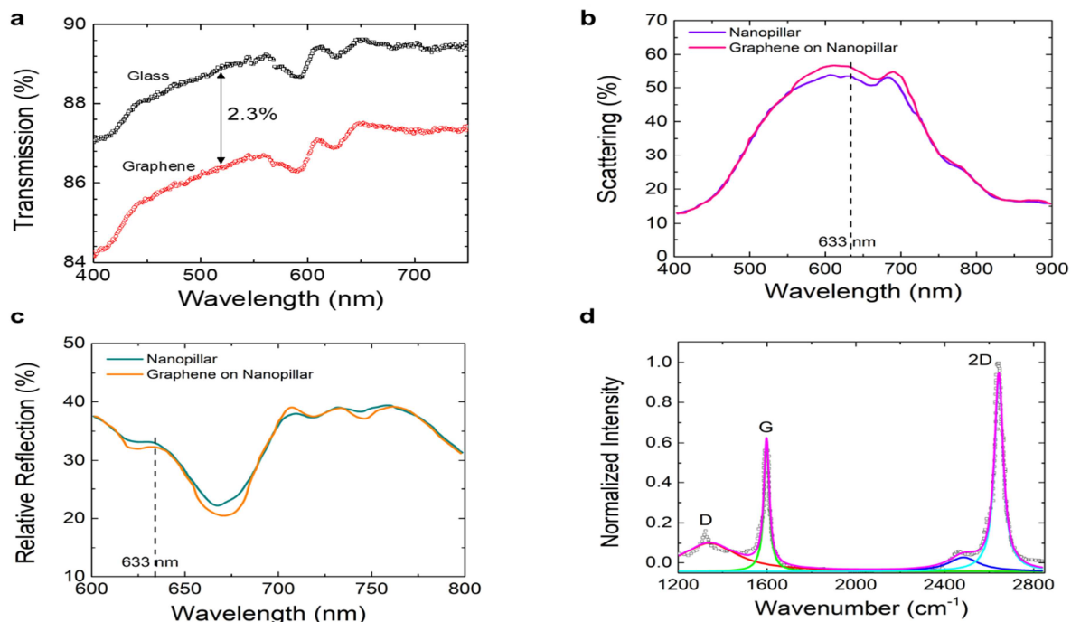
Figure 2. Optical properties of graphene covered Au@Ag core-shell nanopillars SERS substrate. (a) Transmission spectra. (b) Scattering spectra. (c) Reflection spectra. (d) Measured Raman spectra of the single-layer of graphene on the SERS substrate. The Lorentzian fits of the full spectra (pink line) and the corresponding fit to individual D (red), G (green) and 2D (cyan) bands are shown.
