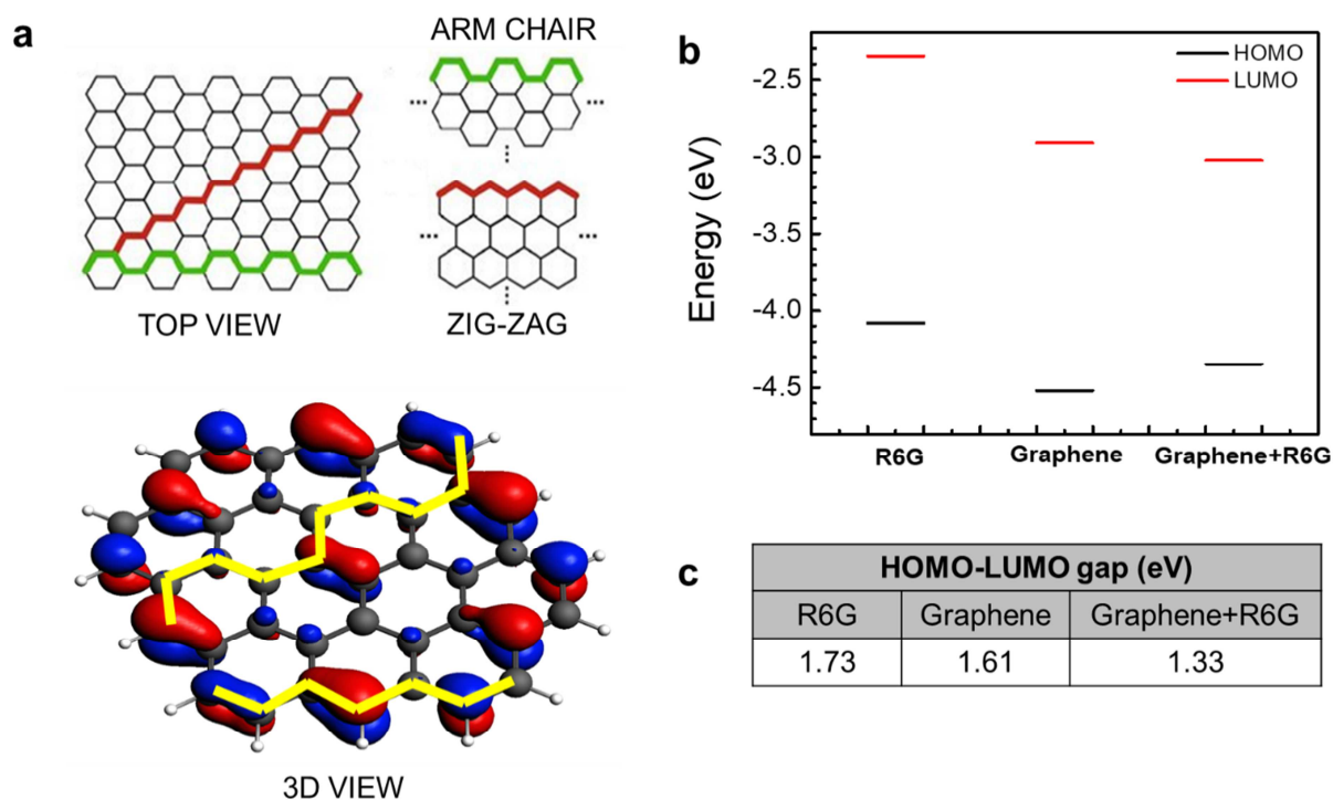
Figure 7. (a) Optimized geometry of graphene using Density Functional Theory (DFT). High electron density along the zig-zag (trans) edge compared to arm chair (cis) is shown. The inset shows the schematic of the arm chair (green) and zig-zag (red) configuration of graphene edge. (b) Position of HOMO and LUMO energy level and (c) HOMO-LUMO band gap for R6G, Graphene and R6G conjugated graphene.
