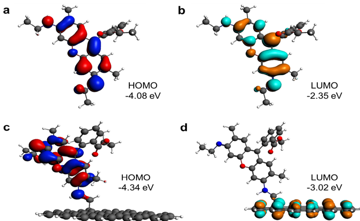
Figure 8. Electron density plot showing the (a) HOMO and (b) LUMO level for R6G before adsorption to graphene. Electron density plot showing the (c) HOMO and (d) LUMO level for R6G after adsorption to graphene.
