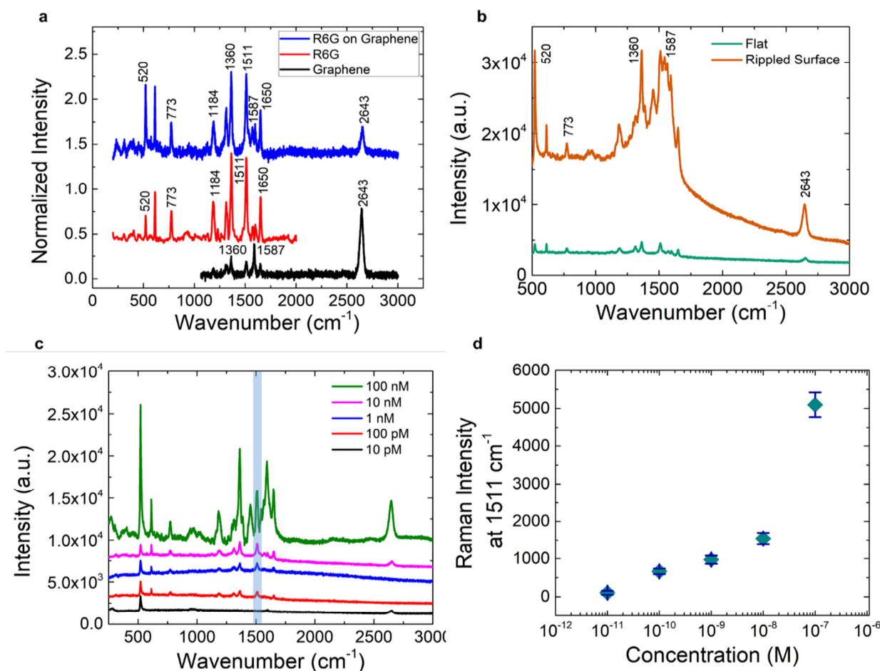
Figure 3. (a) Raman spectra of R6G on graphene coated nanostructured SERS substrate (blue line (100 nM)), bulk R6G (red line (1 μM)) and single layer graphene on flat surface (black line). (b) Evaluation of enhancement factor from surface enhanced Raman spectroscopy (SERS) substrate in comparison to flat surface. The corresponding concentrations are C_{(flat)bulk} = 100 \mu\text{M} and C_{(rippled)SERS} = 100 \text{nM} . (c) SERS spectra of R6G on the Au@Ag core-shell substrate at concentrations ranging from 10 pM to 100 nM. (d) SERS intensity as a function of concentration at the 1511 cm -1 Raman peak.
