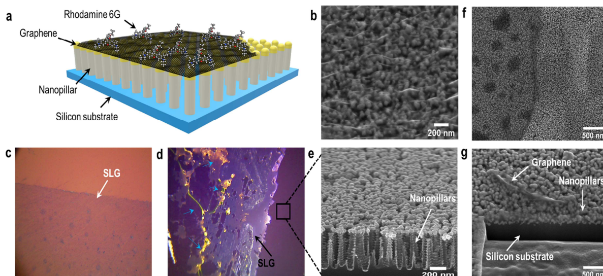
Figure 1. (a) Schematic diagram showing graphene ripple on the plasmonic nanopillar SERS substrate. (b) Scanning Electron Micrographs (SEM) of graphene on the SERS substrate. (c, d) Optical image of graphene on the SERS substrate. Rhodamine 6G (R6G) is appearing as yellow in the image (shown by blue arrows). (e) Vertical cross-sectional SEM image of the Au@Ag core-shell nanopillars taken from the black square region of image shown in (d). (f) SEM image showing graphene over the 10\ \mu\text{m} \times 10\ \mu\text{m} area of the substrate. (g) Focused Ion Beam (FIB) cut area showing the cross-sectional view of graphene, Ag coated Au nanopillar, and silicon substrate.
