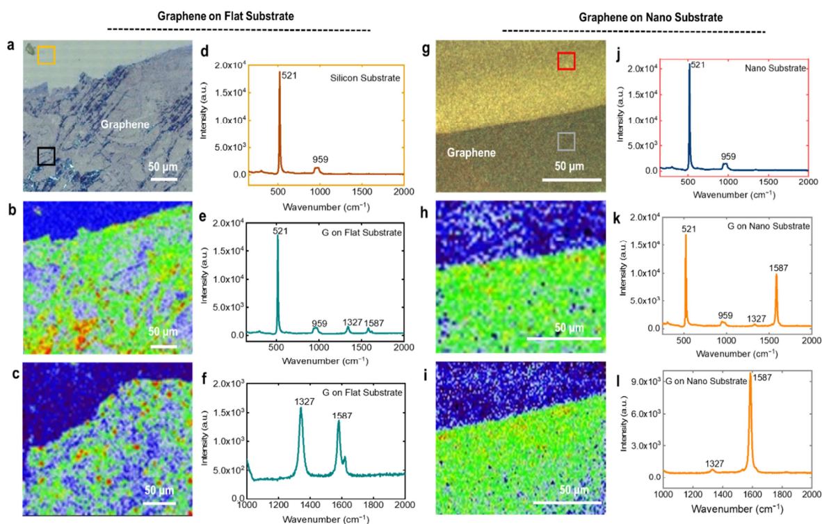
Figure 4. Representative bright field images of (a) graphene on flat substrate, and (g) graphene on nanostructured substrate. Raman mapping of graphene on flat substrate (b) using 532 nm laser excitation; magnification: 50X; number of acquired spectra: 25017), and (c) using 633 nm laser excitation; magnification: 50X; number of acquired spectra: 14012). Raman spectra on (d) silicon substrate (orange square highlighted area shown at the inset of (a)), (e) graphene on flat substrate (black square highlighted area shown at the inset of (a)), (f) zoomed in spectral region from 1000-2000 cm -1 shown in Figure 4e . Raman mapping of graphene on nano substrate (h) using 532 nm laser excitation; magnification: 50X; number of acquired spectra: 10850), and (i) using 633 nm laser excitation; magnification: 50X; number of acquired spectra: 10850). Raman spectra on (j) nano substrate (red square highlighted area shown at the inset of (g)), (k) graphene on nano substrate (black square highlighted area shown at the inset of (g)), (l) zoomed in spectral region from 1000-2000 cm -1 shown in Figure 4k .
