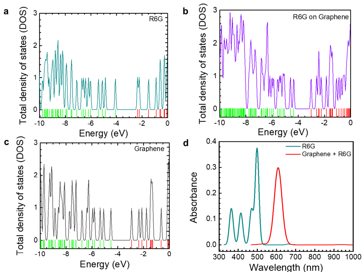
Figure 9. Distribution of total density of states (DOS) for (a) R6G, (b) R6G on graphene, and (c) graphene showing the occupied (green) and unoccupied (red) molecular orbitals. The Fermi level is set as 0 eV. (d) Theoretical absorption spectrum (DFT) of R6G and R6G adsorbed on graphene.
