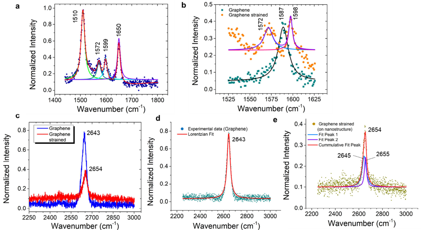
Figure 5. Raman spectra of R6G on graphene coated nanostructured substrate showing the (a) experimental data (blue diamonds), and Lorentzian fits. The overall fit is shown with the red line. (b) Comparison of G peak for unstrained graphene (on flat surface) and strained graphene (on nanostructured surface leading to ripple). The splitting of G peak shows that the graphene is under strain on the nanostructured surface. (c) Comparison of 2D peak for unstrained graphene (blue line) and strained graphene. The corresponding Lorentzian fits to the experimental data are shown in (d) for unstrained graphene, and in (e) for strained
