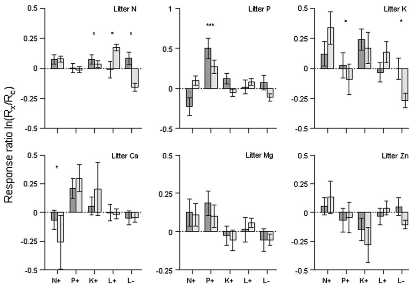
Figure 3. Changes in litter nutrient concentrations in response to fertilization and litter manipulation treatments in old-growth lowland tropical forest in Panama, Central America, expressed as log response ratios relative to controls; dark gray bars show effects after 3 years of treatments and light gray bars show effects after 5 years of treatments; marginally significant effects ( P < 0.1 ) are denoted by °; see Figure 1 for a description of other symbols and abbreviations.
